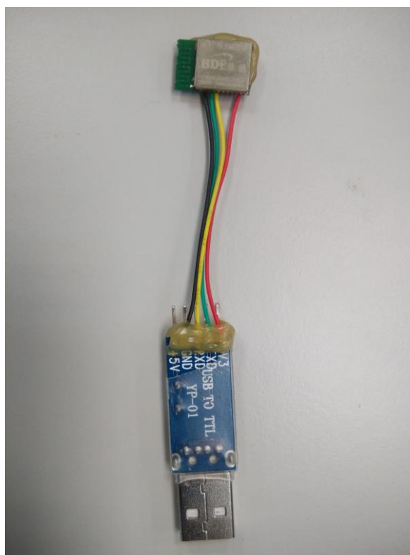
BT cable for Model 2(BT)
